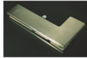
Model: BPF-004 Item: Big clamp for over panel & side panel Finish: SN MRP: Rs.2,820 per pc
